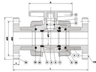
FLANGE TYPE
